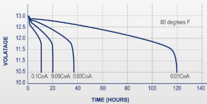
Discharge characteristics
